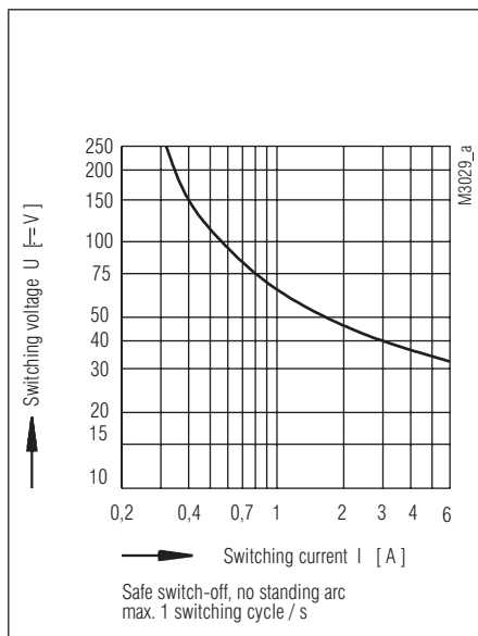
Limit curve for arc-free operation (at t_u = 20^\circ\text{C} )
