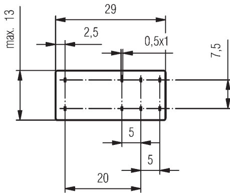
Drilling plan (solder side)
