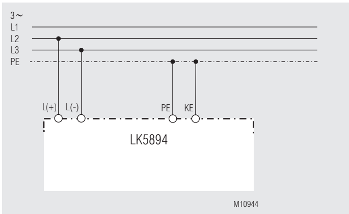
Insulation monitoring AC-side
