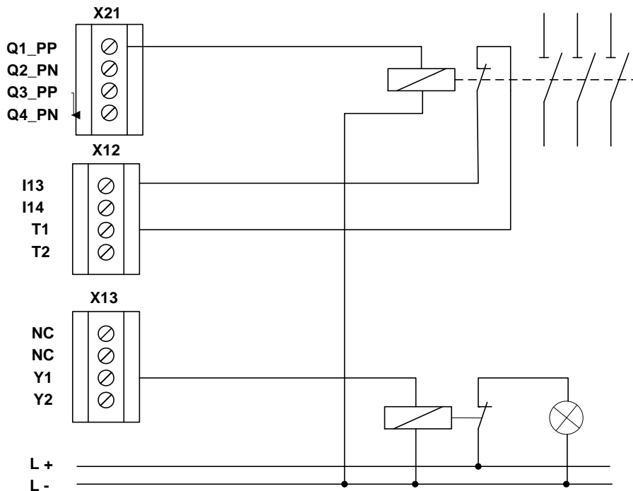
Fig.: Single-channel relay output with testing
