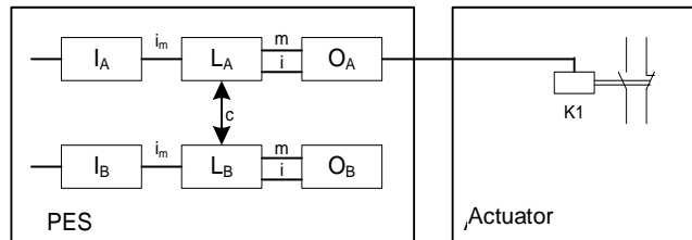
Single-channel output SMX and single-channel actuator without diagnostics
