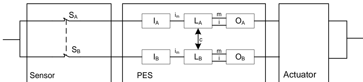
Two-channel input element in parallel connection (Cat. fault tolerance 1) with high DC caused by signal in two channels and diagnose by means of cross-comparison in the PES
