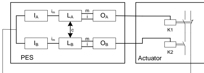
Dual-channel output SMX and dual-channel actuator with single-channel diagnose
