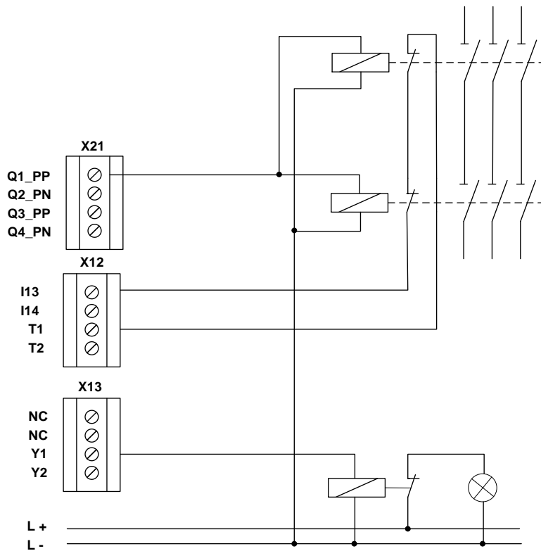
Fig.: Single-channel switching outout Q1_PP with dual-channel external circuit and monitoring at output 13 1 as group feedback
