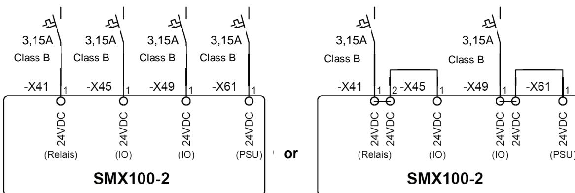
Connection example with separate IO supply! (when connecting IO's with high current consumption)
