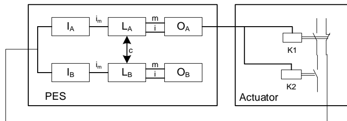
Single-channel output SMX (Q 5/6, Q 1/3, Q 2/4) and dual-channel actuator with at least single-channel diagnostics.
