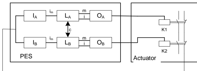
Dual-channel output SMX and dual-channel actuator with dual-channel diagnose
