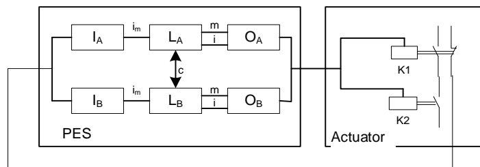
Single-channel output SMX with internal dual-channel processing (IQQ x) and dual-channel actuator with at least single-channel diagnose
