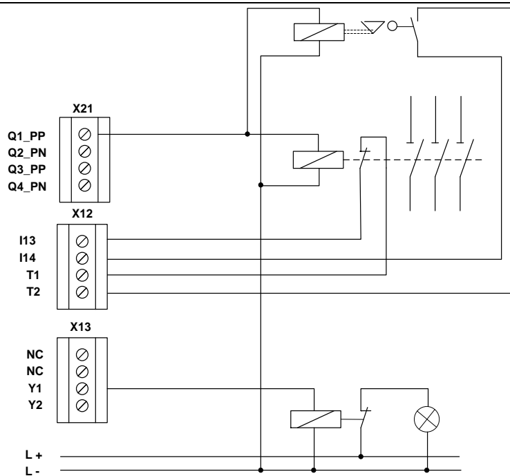
Fig.: Single-channel switching output Q1_PP with dual-channel external circuit as combination of electro-mechanical element and hydraulic/pneumatic valve and monitoring at two inputs
