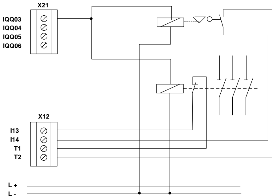
Fig.: Two-channel output in connection with two-channel switching-off circuit with testing
