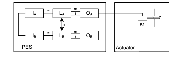
Single-channel output SMX and single-channel actuator with diagnostics
