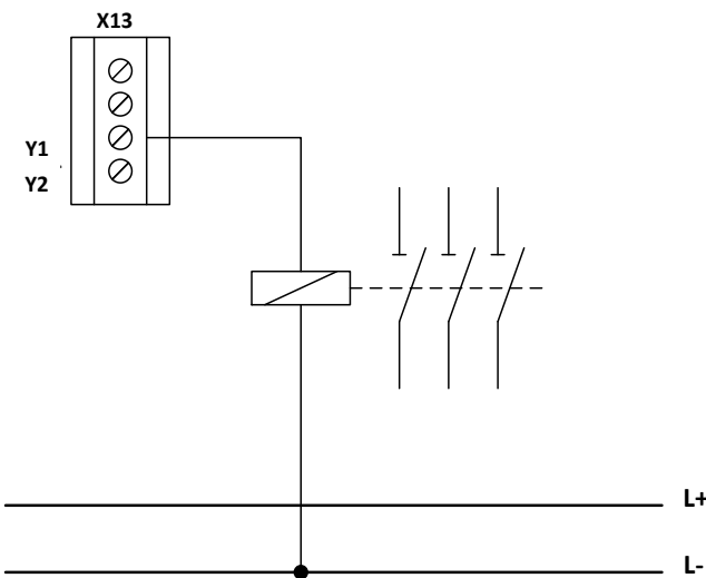
Fig.: Wiring of a notification output
