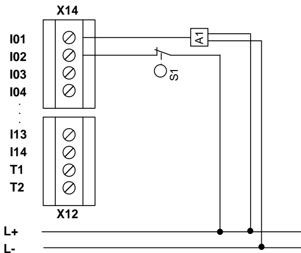
Figure: dual-channel input element heterogeneous, without cycling
