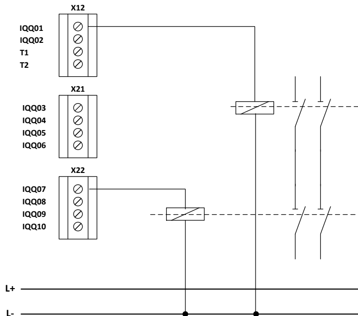
Fig.: Redundant two-channel outputs in different groups in connection with two-channel switching-off circuit
