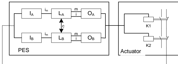
Single-channel output SMX with internal dual-channel processing (IQQ x) and dual-channel actuator with dual-channel diagnose
