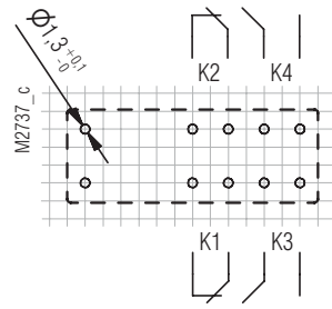
OA5670.52__L1 2NO/2NC
