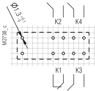
OA5670.48__L1 3NO/1NC
