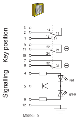
Fig. 1: Locked while activated: 1st key removed, Actuator inserted, 2nd key inserted, Door closed
