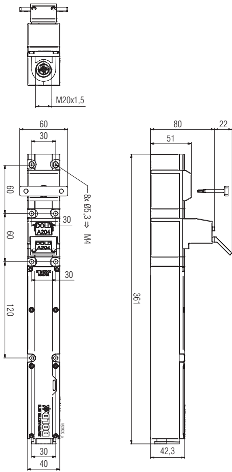
YRX10BM/K Clearance tolerances ± 2%
