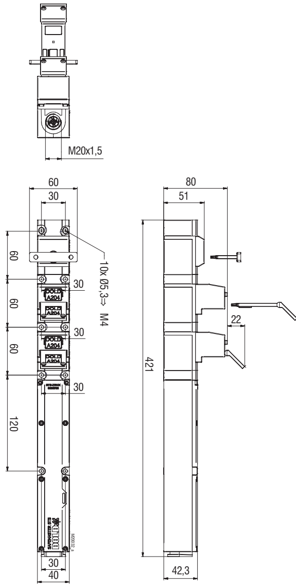
YRX11BM/K Clearance tolerances ± 2%
