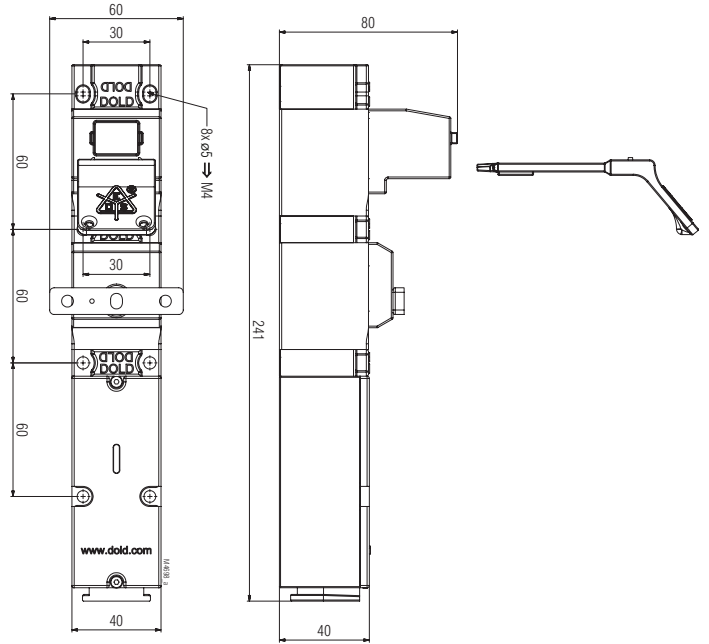
RXK01M Clearance tolerances ± 2%
