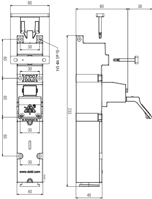
RX10A Clearance tolerances ± 2%
