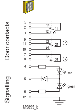
Fig. 2: Locked while activated: Actuator inserted, 2nd key inserted, 1st key removed, door closed
