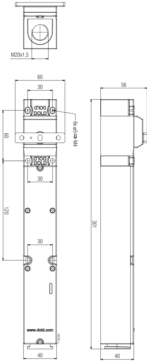
Illustrations: YRXKM Clearance tolerances ± 2%
