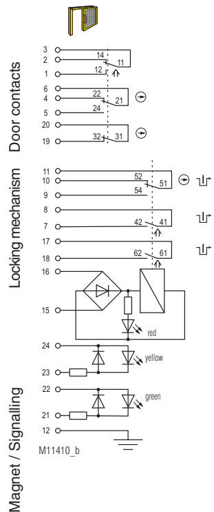
Fig. 1: Solenoid locking activated: Magnet locked, 1st key removed, actuator and 2nd key inserted, Door closed
