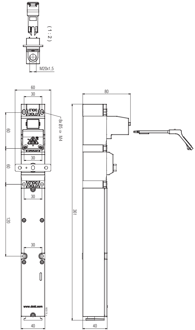
Illustrations: YRXK01M Clearance tolerances ± 2%
