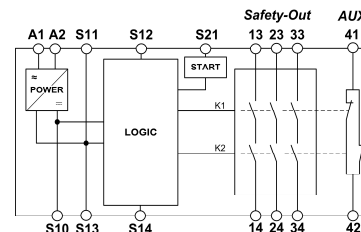
Fig. 1 Block diagram SR3AD
