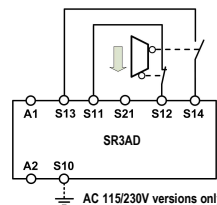
Fig. 5: Dual channel safety guard monitoring with short circuit and ground fault monitoring. (Category 4, up to PL e / SIL 3)
