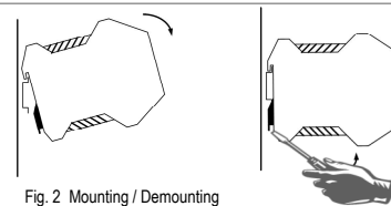
Fig. 2 Mounting / Demounting
