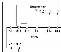
Fig. 4: Two-channel emergency stop circuit with short circuit and earth fault monitoring. (category 4, up to PL e / SIL 3)
