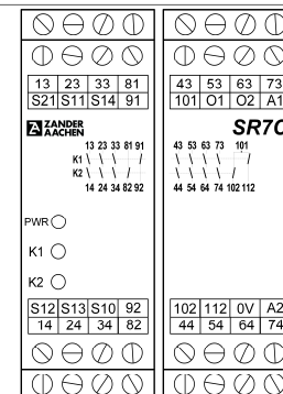
Fig. 3 Connections
