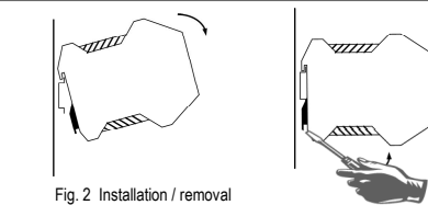
Fig. 2 Installation / removal
