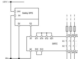
Fig. 9: Connecting to a safety PLC (category 4, up to PL e / SIL 3) Prerequisite: Fault exclusion for cross-circuit (e.g. according to EN ISO 13849-2; Table D4 - wiring in protected wiring space) and PLC also meets requirements for category 4, PL e / SIL 3.
