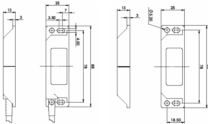
ZCode-LR switch (left) and actuator (right)
